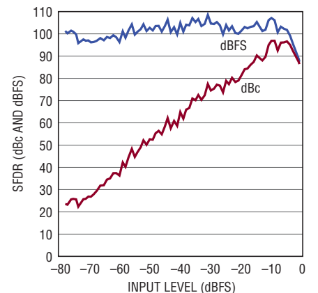
LTC2141-12: SFDR vs Input Level, f_{IN} = 70\text{MHz} , 40\text{Msps} , 2\text{V} Range
