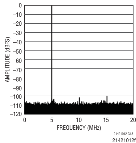
LTC2141-12: 64k Point FFT, f_{IN} = 5\text{MHz} , -1dBFS, 40Msps
